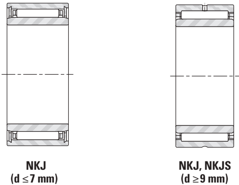
TYPES OF BEARINGS Needle roller bearings with inner rings
