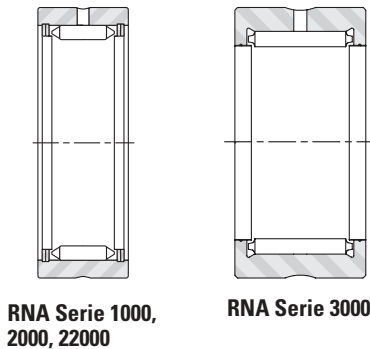
Needle roller bearings without inner rings
