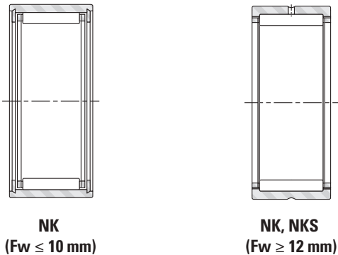
Needle roller bearings without inner rings
